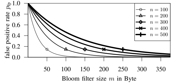
Fig. 2. False positive rate p_{fp} vs. Bloom filter size m for increasing numbers of inserted elements n .
