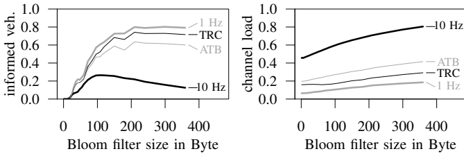
(e) Fraction of informed 2-hop neighbors vs. Bloom filter size incorporating non-symmetric nodes. (f) Wireless channel utilization vs. Bloom filter size incorporating non-symmetric nodes.
