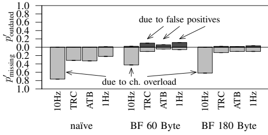
(a) Freeway: Fraction of missing and outdated 1-hop neighbors.
