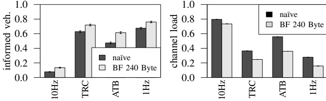
(c) Fraction of informed 2-hop neighbors using a fitting Bloom filter size. (d) Wireless channel utilization using a fitting Bloom filter size.
