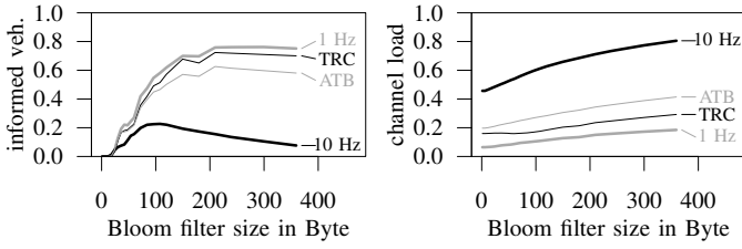
(a) Fraction of informed 2-hop neighbors vs. Bloom filter size. (b) Wireless channel utilization vs. Bloom filter size.
