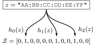
Fig. 1. Adding an element z (here, a MAC address) to an initially empty Bloom filter \mathcal{Z} (of size m = 12 bit and using k = 3 hash functions).
