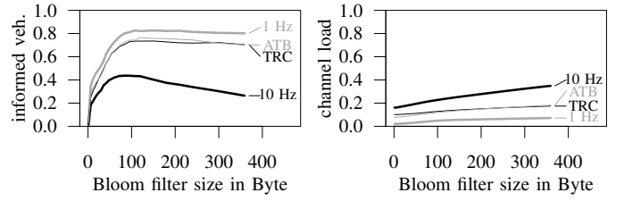
(a) Fraction of informed 2-hop neighbors vs. Bloom filter size. (b) Wireless channel utilization vs. Bloom filter size.
