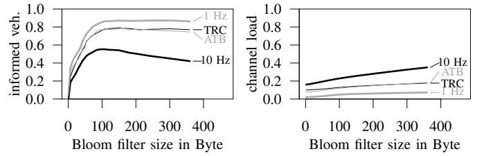
(e) Fraction of informed 2-hop neighbors vs. Bloom filter size incorporating non-symmetric nodes. (f) Wireless channel utilization vs. Bloom filter size incorporating non-symmetric nodes.
