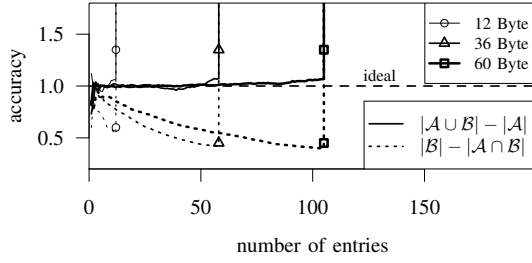
Fig. 4. Estimation accuracy for the number of additional entries provided by a certain Bloom filter normalized to the ground truth. The line width depicts the Bloom filter size; dotted and solid lines represent the two calculation options.
