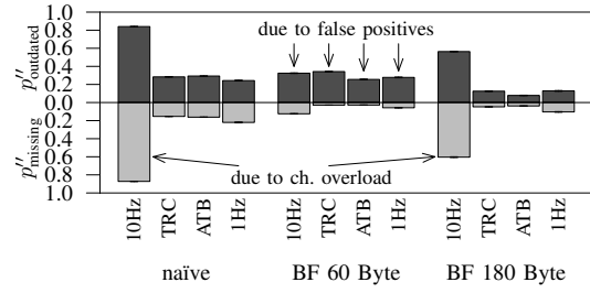
(b) Freeway: Fraction of missing and outdated 2-hop neighbors.
