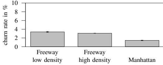
Fig. 6. Neighbor churn rate for different scenarios and traffic densities (average value and 95 % confidence interval).
