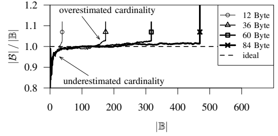
Fig. 3. Estimating the number of inserted elements in a Bloom filter. The line width depicts the Bloom filter size; the dashed line shows the ideal behavior.
