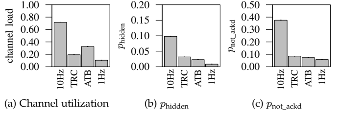
Fig. 5. Beacons performance for the high density freeway scenario (average value and 95 % confidence interval).
